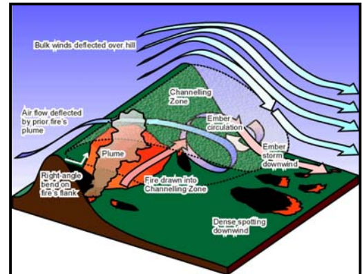
Figure 2. Illustration of a conceptual model for lee-slope channelling
